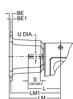
STYLE DM (NEMA MOTORS ONLY)
