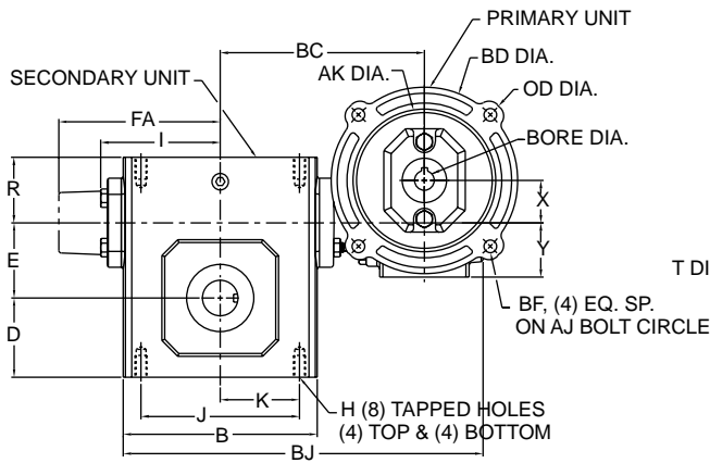
STYLE DMQ (NEMA AND IEC B5 METRIC MOTORS)
