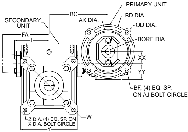
STYLE DFMQ (NEMA AND IEC B5 METRIC MOTORS)
