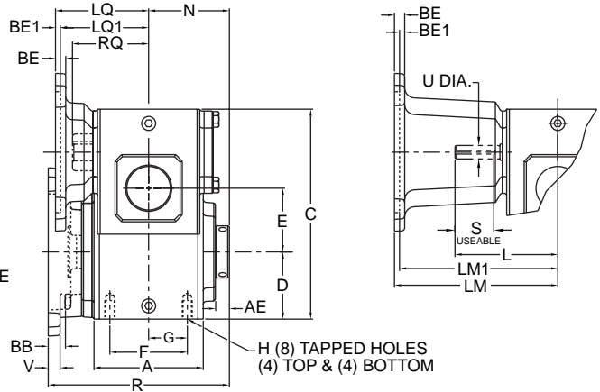
STYLE DFHM (NEMA MOTORS ONLY)
