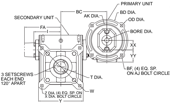
STYLE DFHMQ (NEMA AND IEC B5 METRIC MOTORS)
