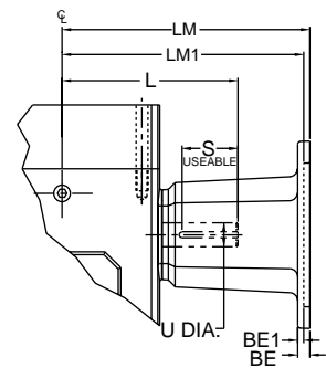
STYLE RM (NEMA MOTORS ONLY)
