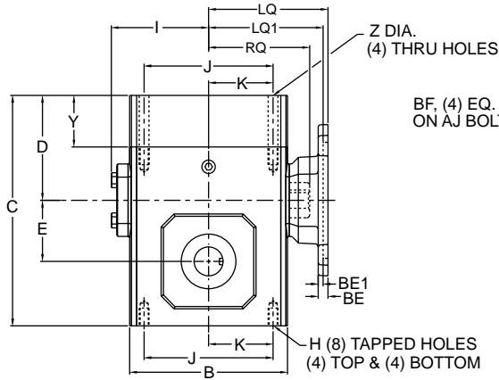
STYLE RMQ (NEMA AND IEC B5 METRIC MOTORS)
